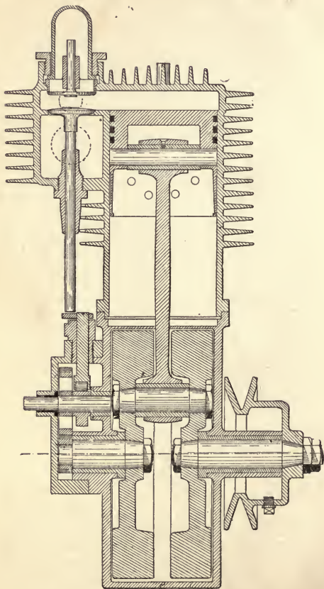
Fig. 34.—Vertical Section of 3\frac{1}{2} -h.p. Petrol Engine.
