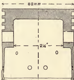
Fig. 39.—Section of Piston on Line X X (Fig. 38).
