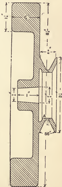
Fig. 127.—Section of Fly-wheel and Pulley.
