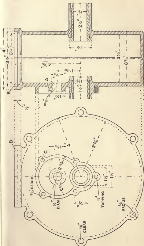
Figs. 53 and 54.—Side Elevation and Vertical Section of Crank Case.
