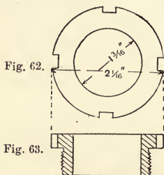
Figs. 62 and 63.—Union Nut.
